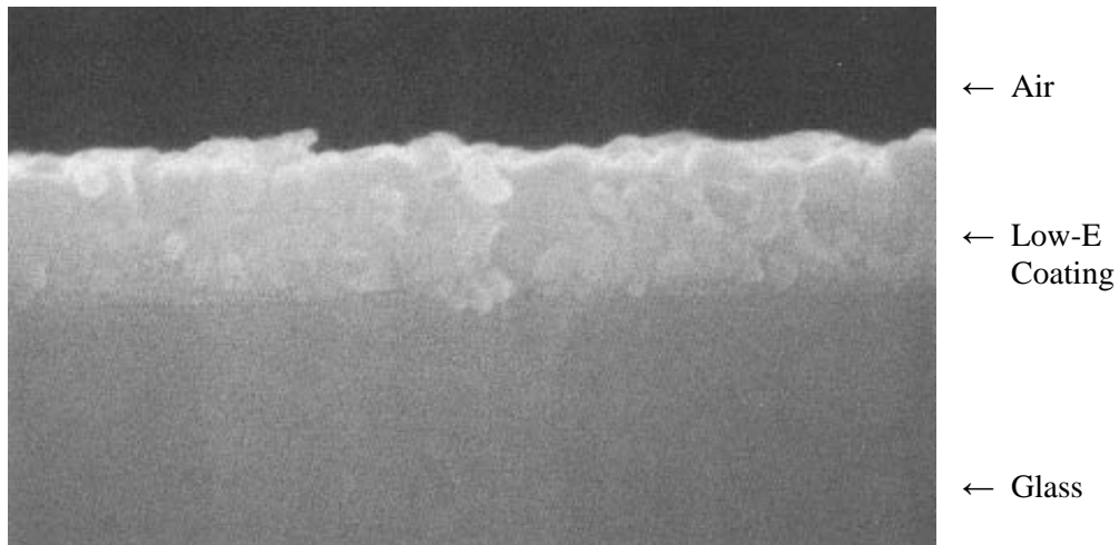
Fig.2. Cross-section showing coating uniformity, magnified 50,000 times.
